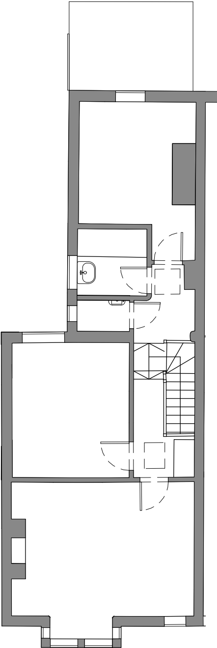
1 Existing First Floor Plan 1:100
