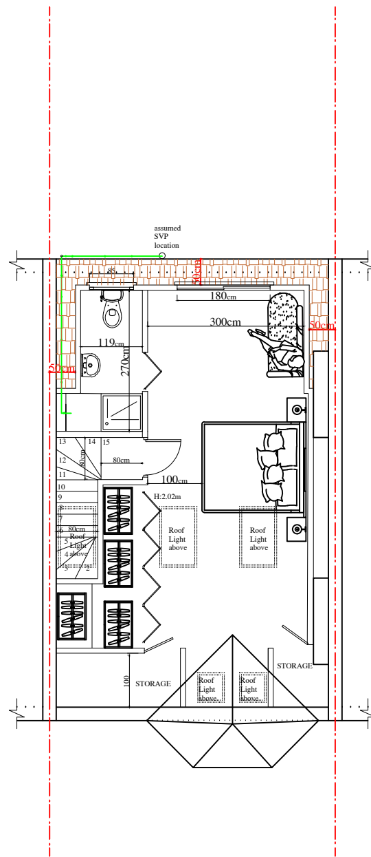
PROPOSED LOFT FLOOR PLAN
