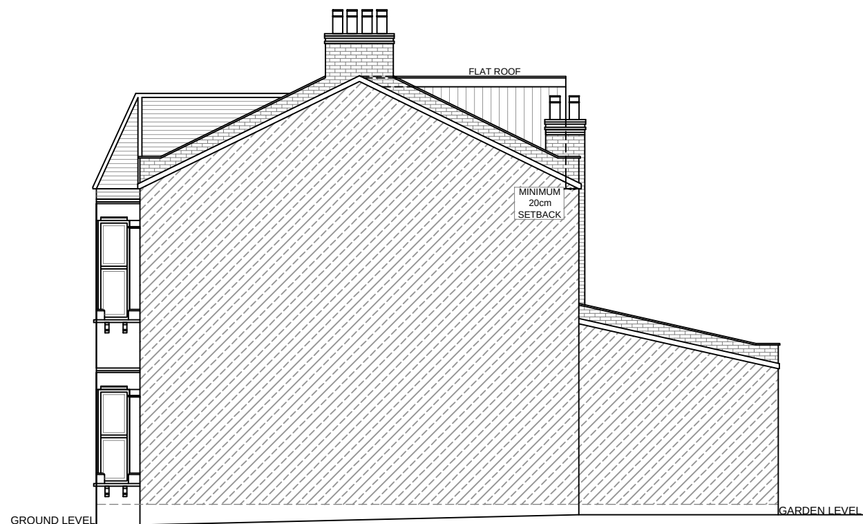
PROPOSED ELEVATION SIDE B
