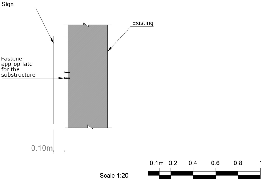
FASCIA SIGN SECTION
