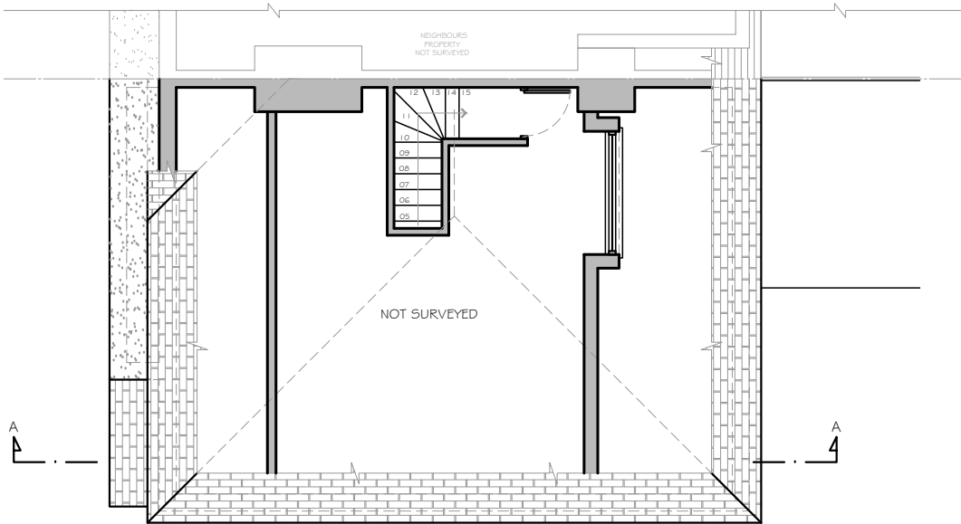
EXISTING LOFT PLAN
