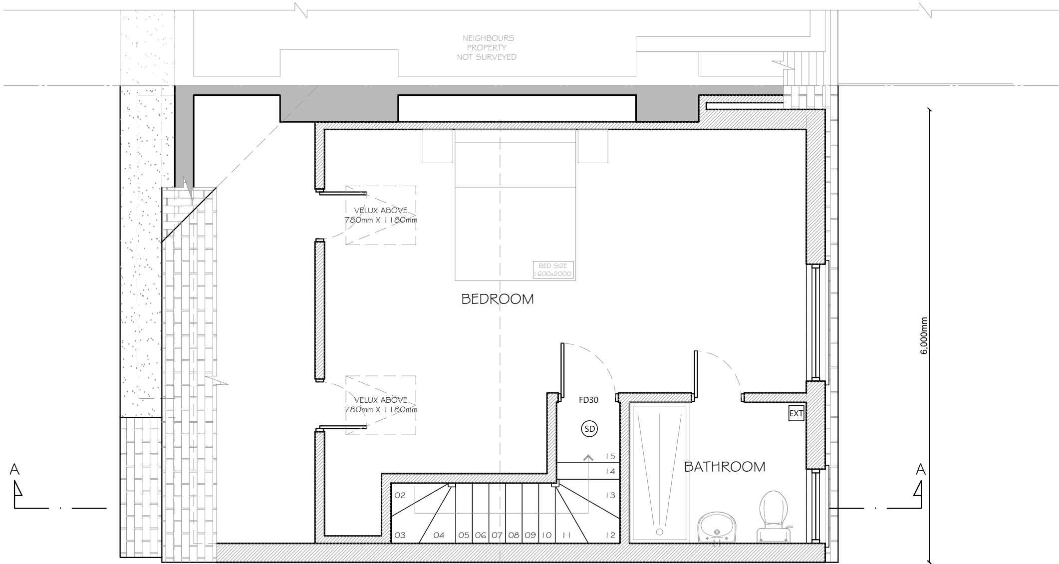
PROPOSED LOFT PLAN
