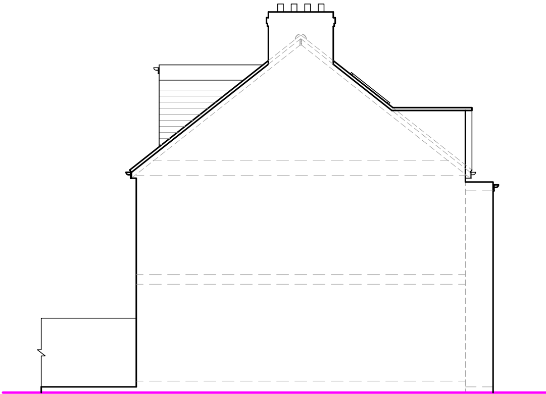
PROPOSED SIDE ELEVATION 02
