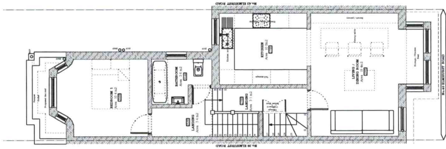
2 Proposed First Floor Plan, Flat 2 CA.00 1:100 @ A3
