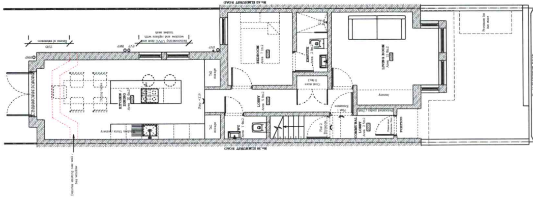
1 Proposed Ground Floor Plan, Flat 1 CA.00 1:100 @ A3
