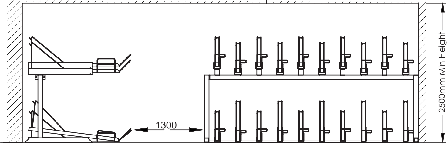
SIDE
