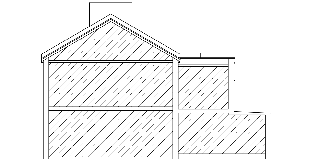
EXISTING SIDE SECTIONAL ELEVATION SCALE 1:100
