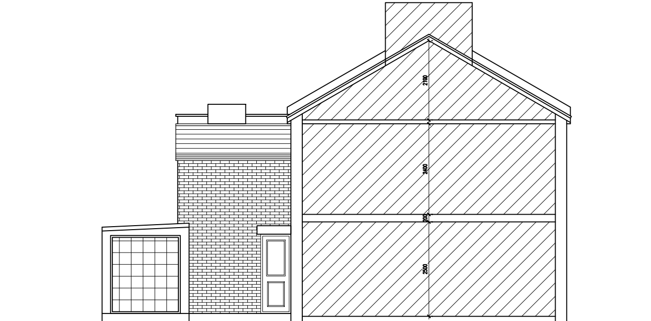
EXISTING SIDE SECTIONAL ELEVATION SCALE 1:100
