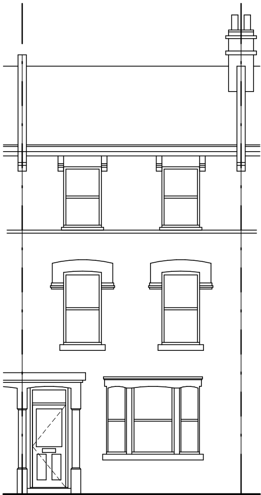
01- Existing Front Elevation
