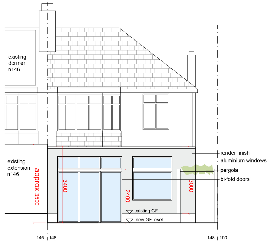
REAR ELEVATION
