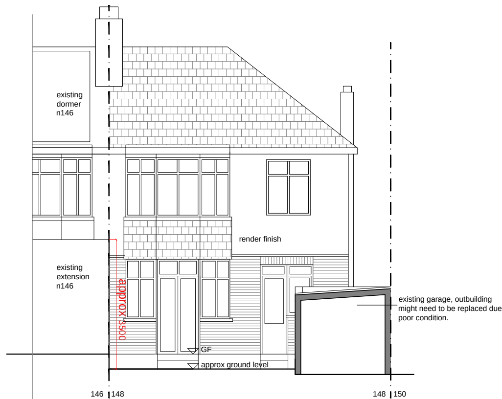
REAR ELEVATION
