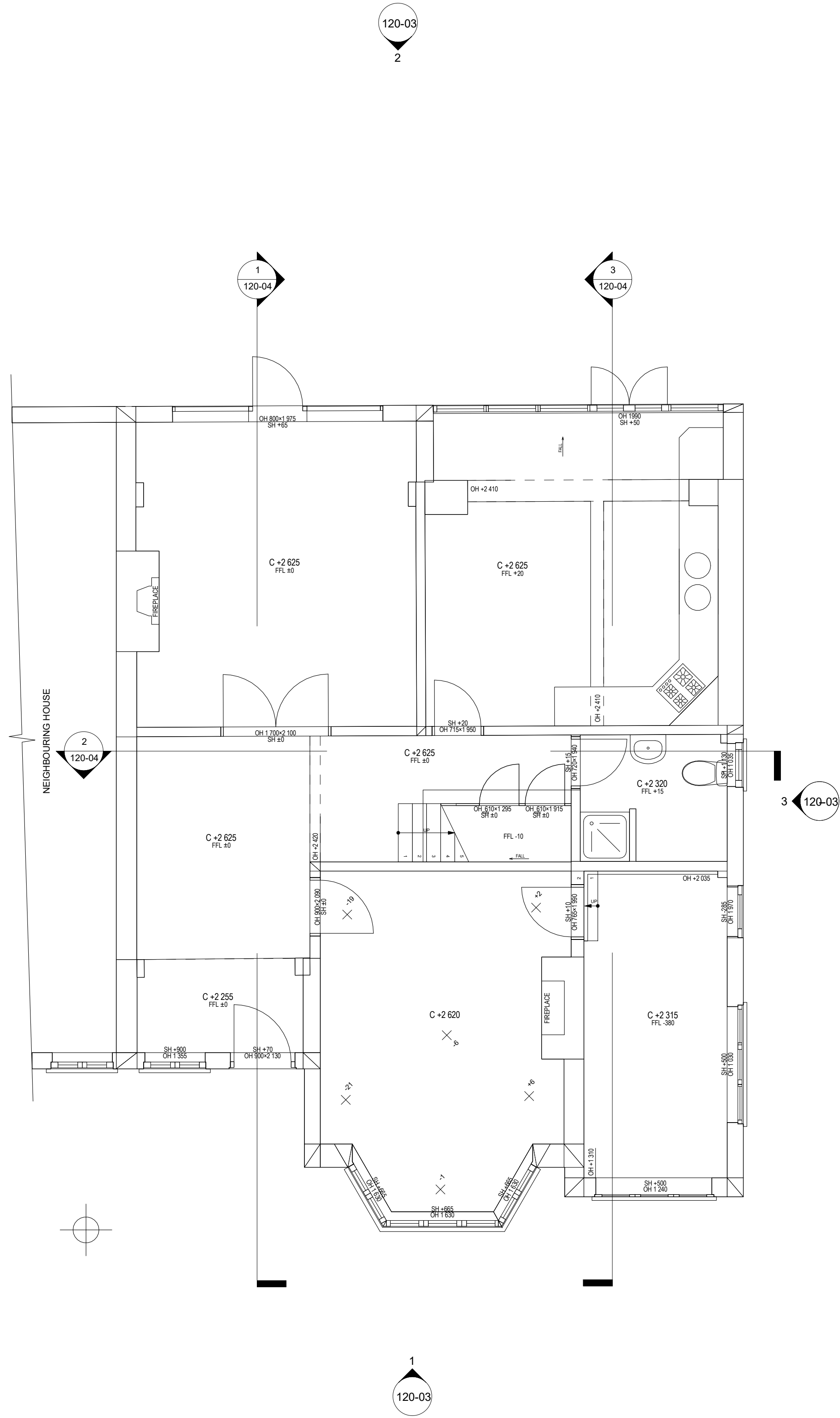
1 Existing Ground Floor 1 : 50
