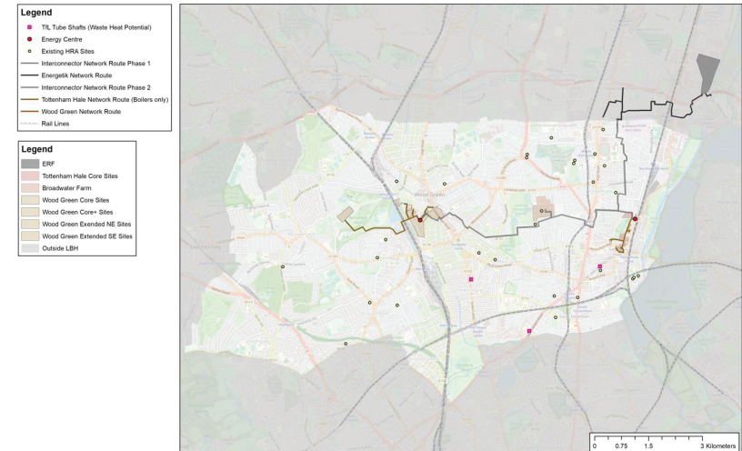
Figure 7-2 District heat network 2023-2025
