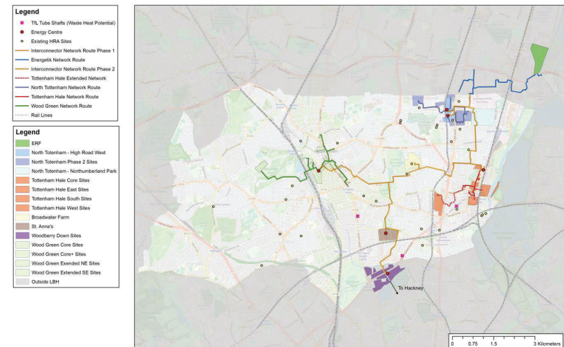
Figure 7-3 District heat network 2030+
