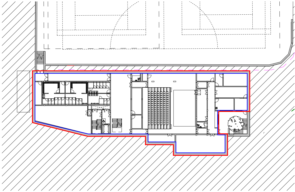
Basement Proposed Area Plan
