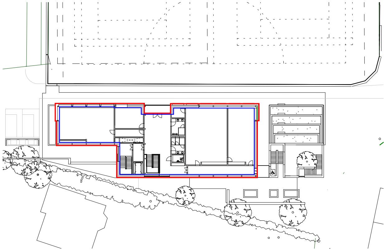
First Floor Proposed Area Plan
