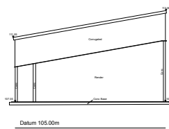
Squash Left Elevation
