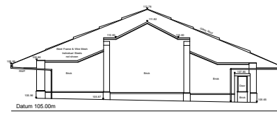
Eton Fives Rear Elevation
