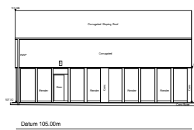
Squash Rear Elevation
