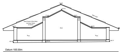
Eton Fives Front Elevation
