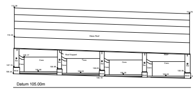
Eton Fives Right Elevation
