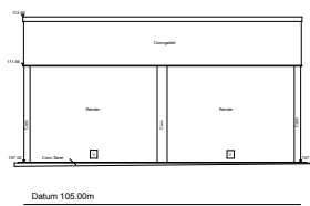
Squash Front Elevation
