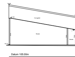
Squash Right Elevation
