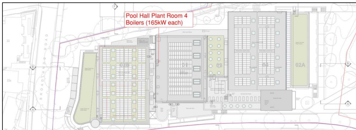
Figure 3 Locations of Boiler Flues – Roof Layout.
