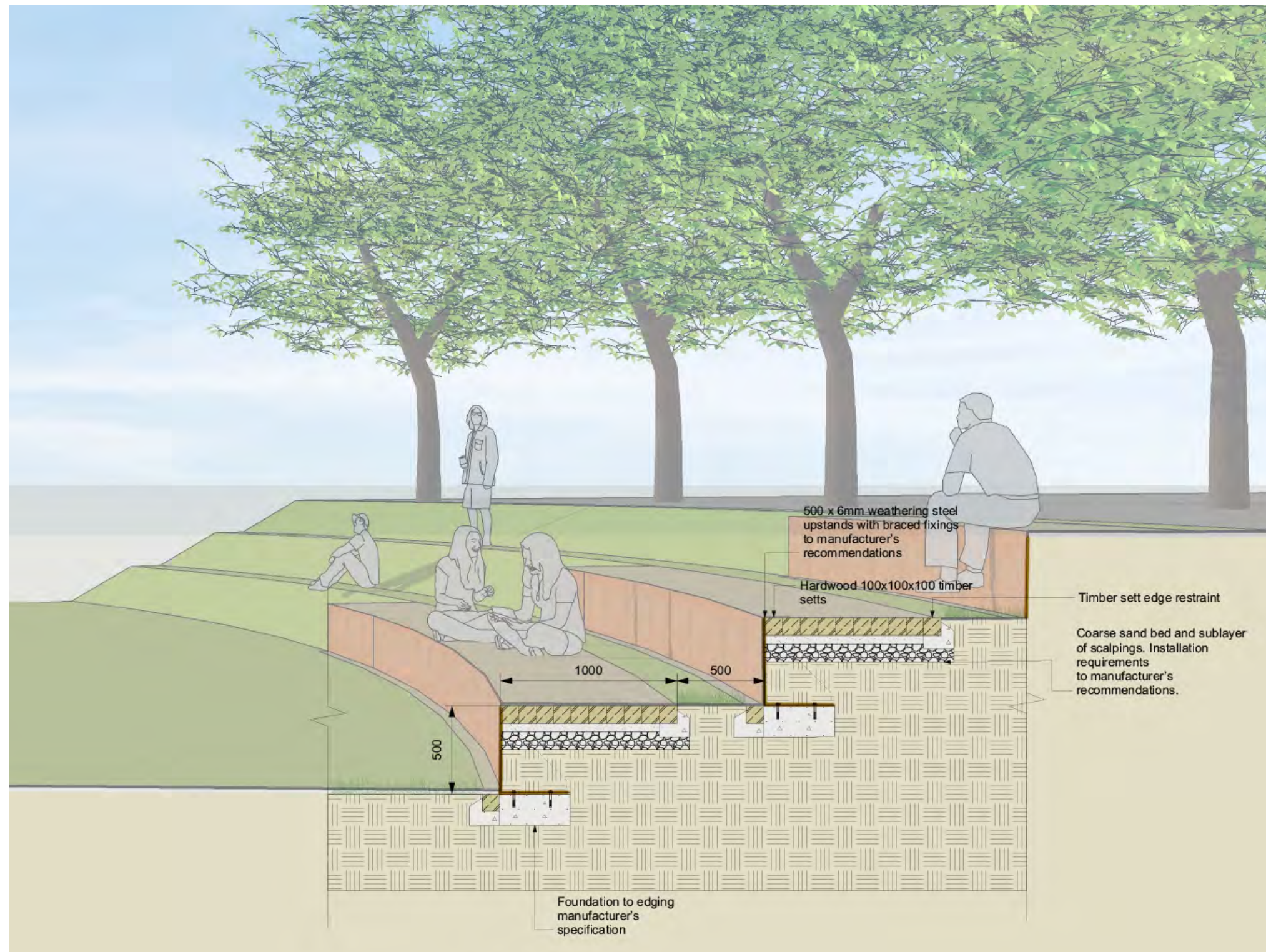
SECTION THROUGH SPORTS PITCH FLOOD BASIN SEATING
