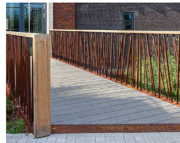
BRIDGE Streetlife timber & corten steel bridge to connect paths besides ancient oak
