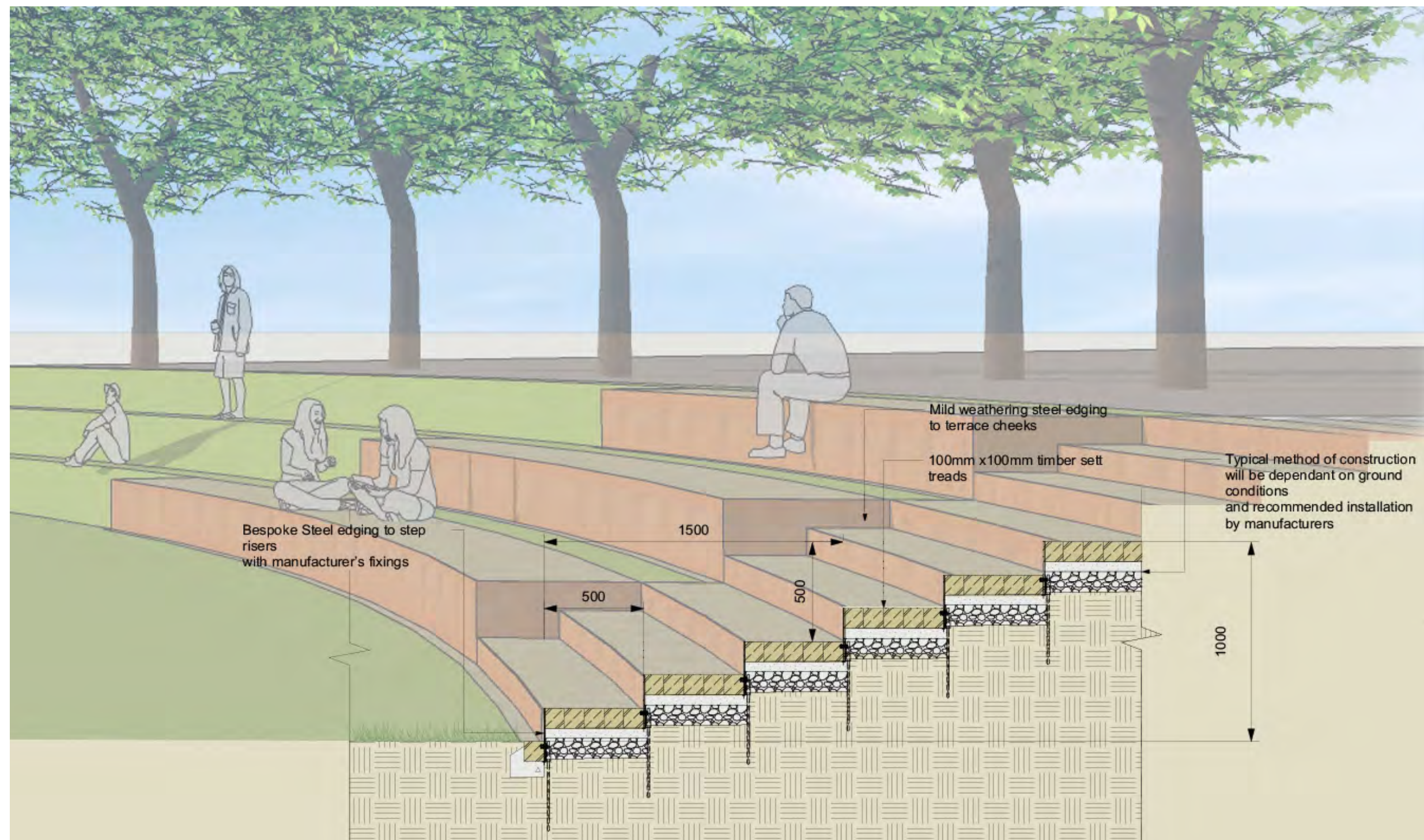
SECTION THROUGH SPORTS PITCH FLOOD BASIN SEATING
