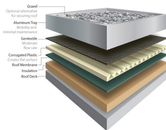
Figure 2: Typical Blue Roof details
