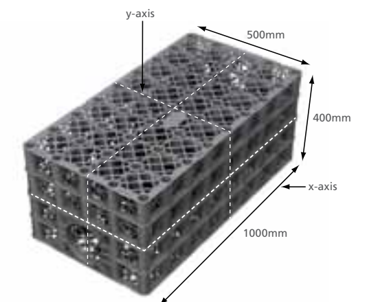
Figure 9 Unit axis; direction of applied load
