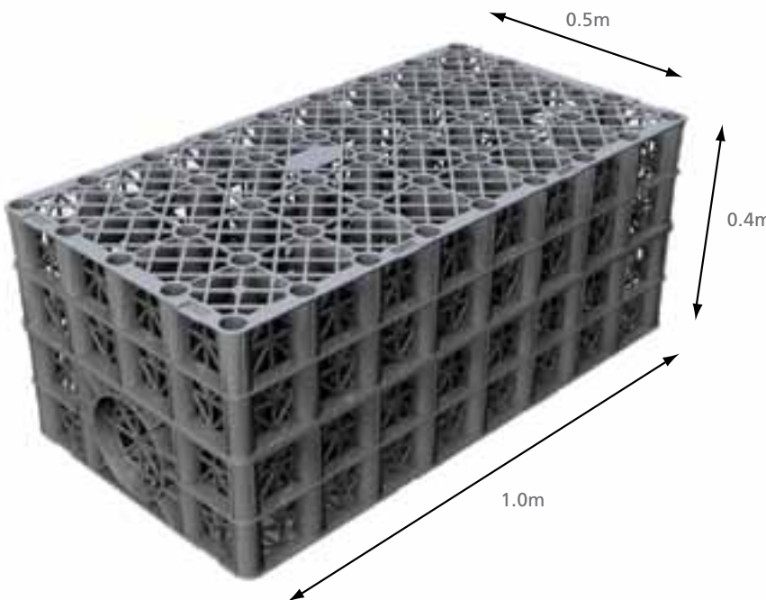
Figure 13 Dimensions of Polystorm cell
