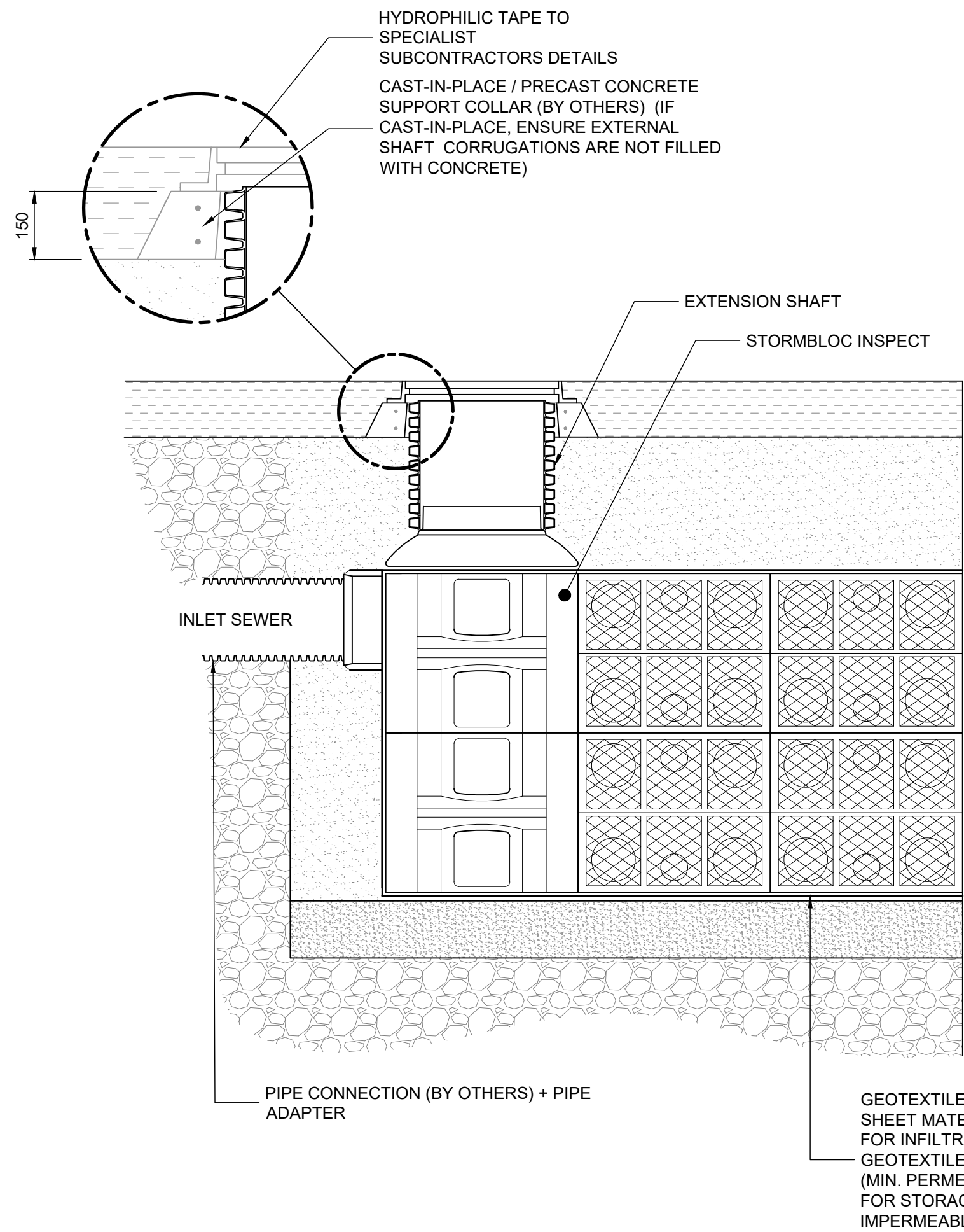
STORMBLOC STORAGE SYSTEM
