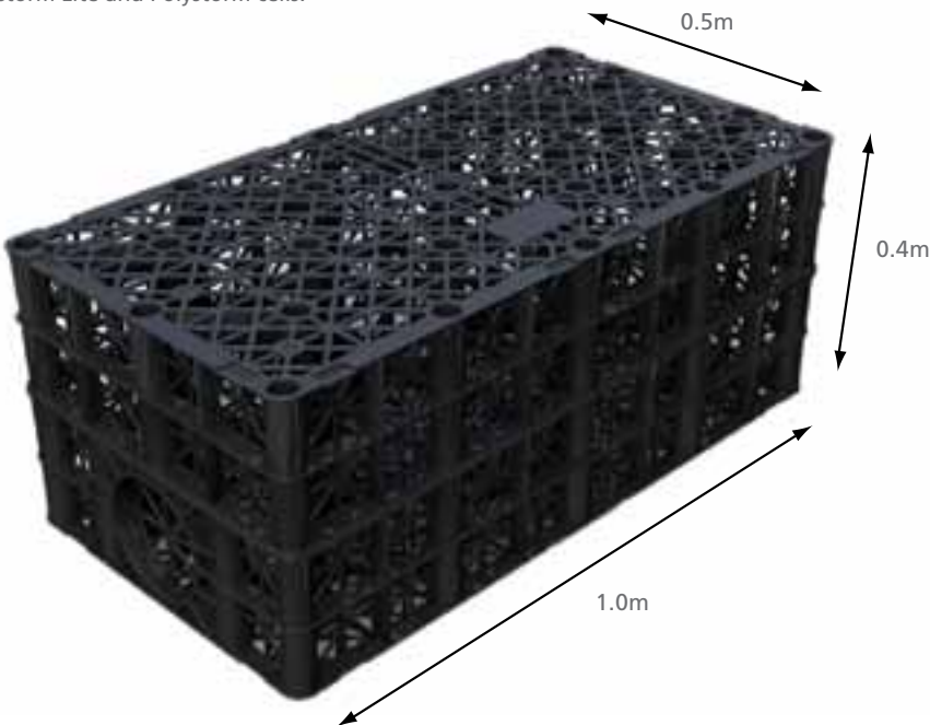
Figure 12 Dimensions of Polystorm Lite cell
