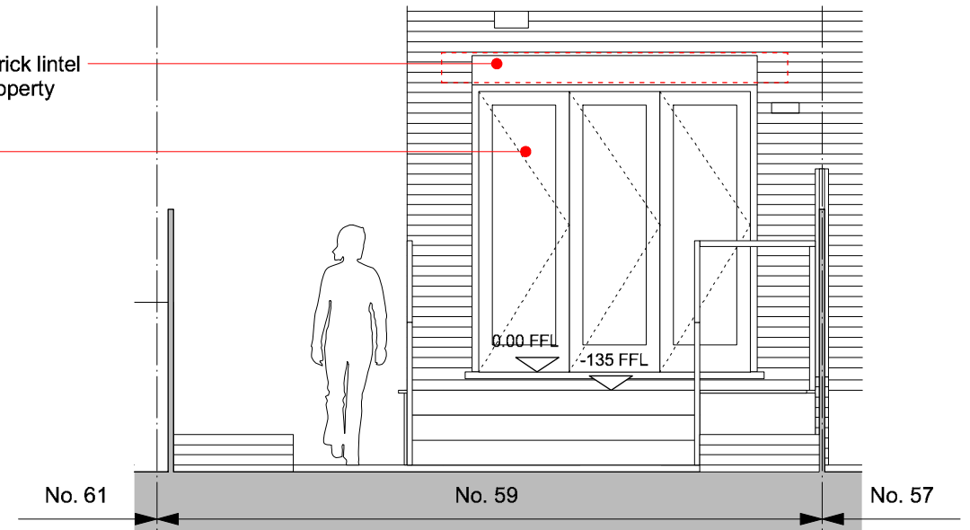
1 Proposed Part Elevation Scale: 1:50
