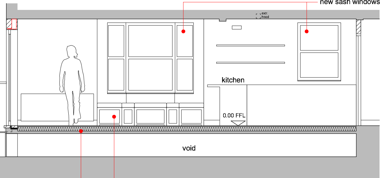
1 Proposed Part Elevation Scale: 1:50
