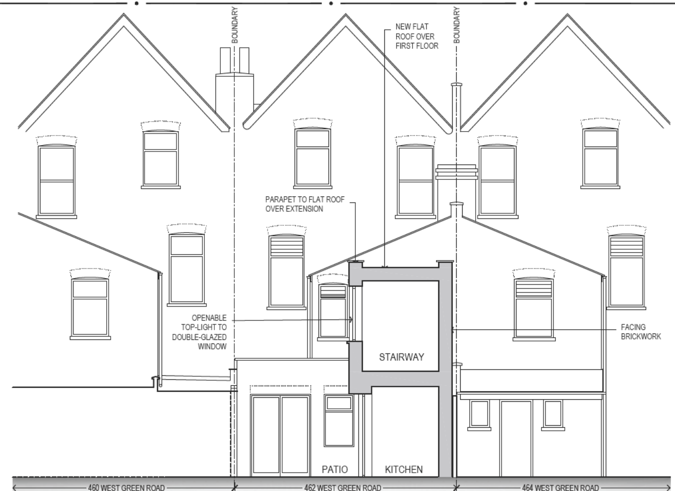
02 Proposed Rear Elevation/Section 1:100@A3 1:50@A1 WEST GREEN ROAD/A/AP243001
