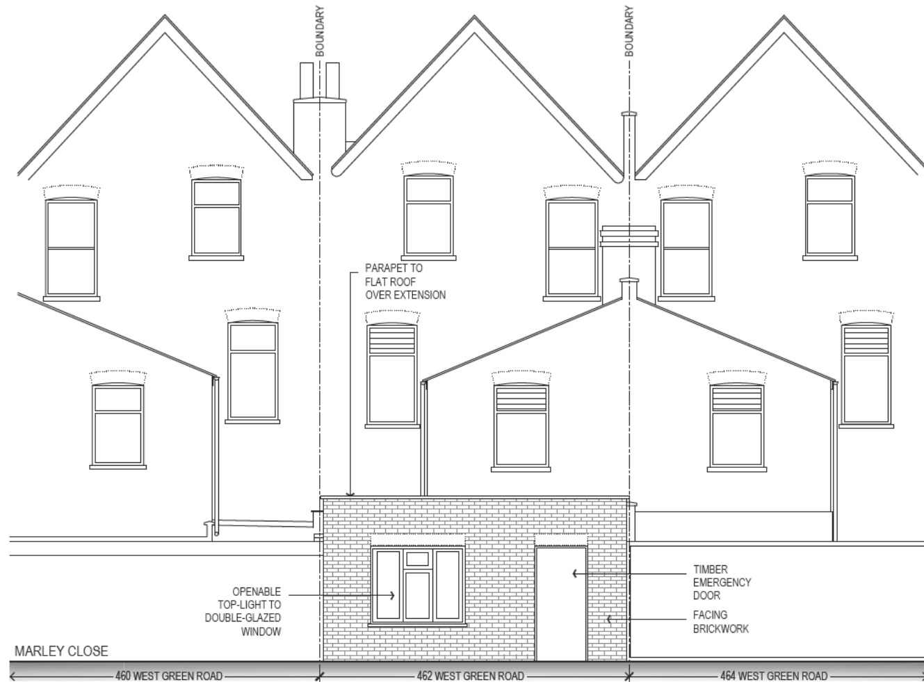
01 Existing Rear Elevation 1:100@A3 1:50@A1 WEST GREEN ROAD/A/AP243001
