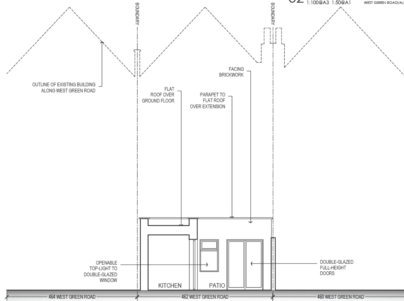
02 Existing Rear Elevation/Section 1:100@A3 1:50@A1 WEST GREEN ROAD/A/AP243001
