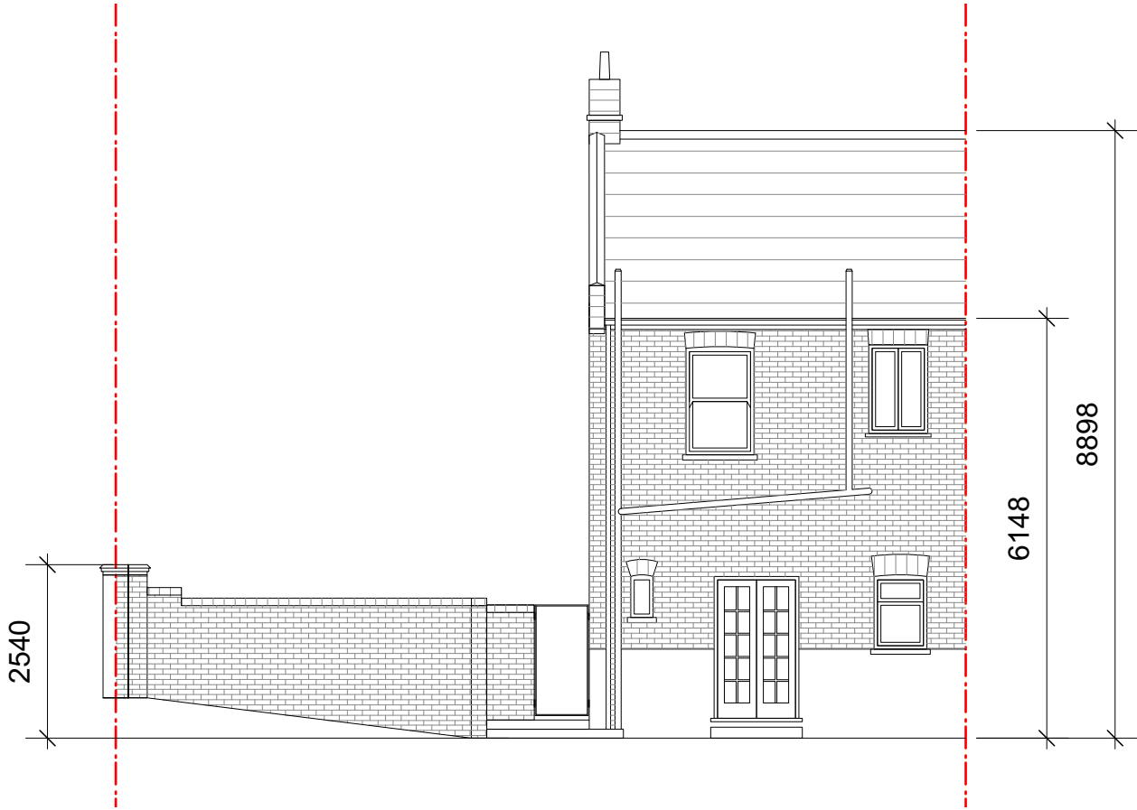
Existing Rear Elevation (south)
