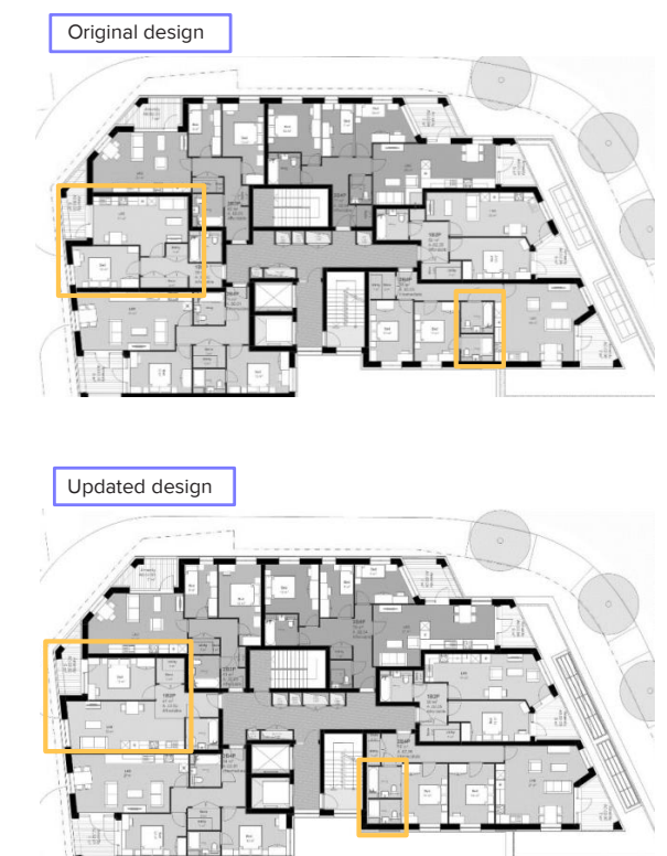
Figure 2: Demonstration of change in layouts to allow for better daylight penetration
