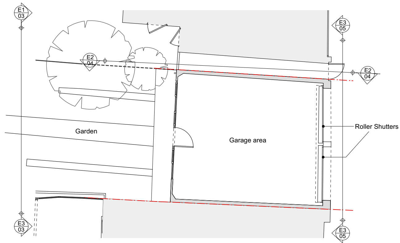
01 - Existing Garage Plan
