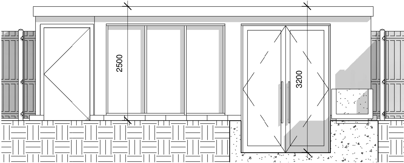
2 Front Elevation 1 : 50
