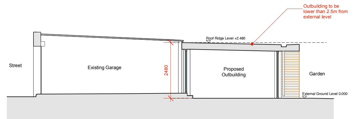
04 - Proposed Section A-A
