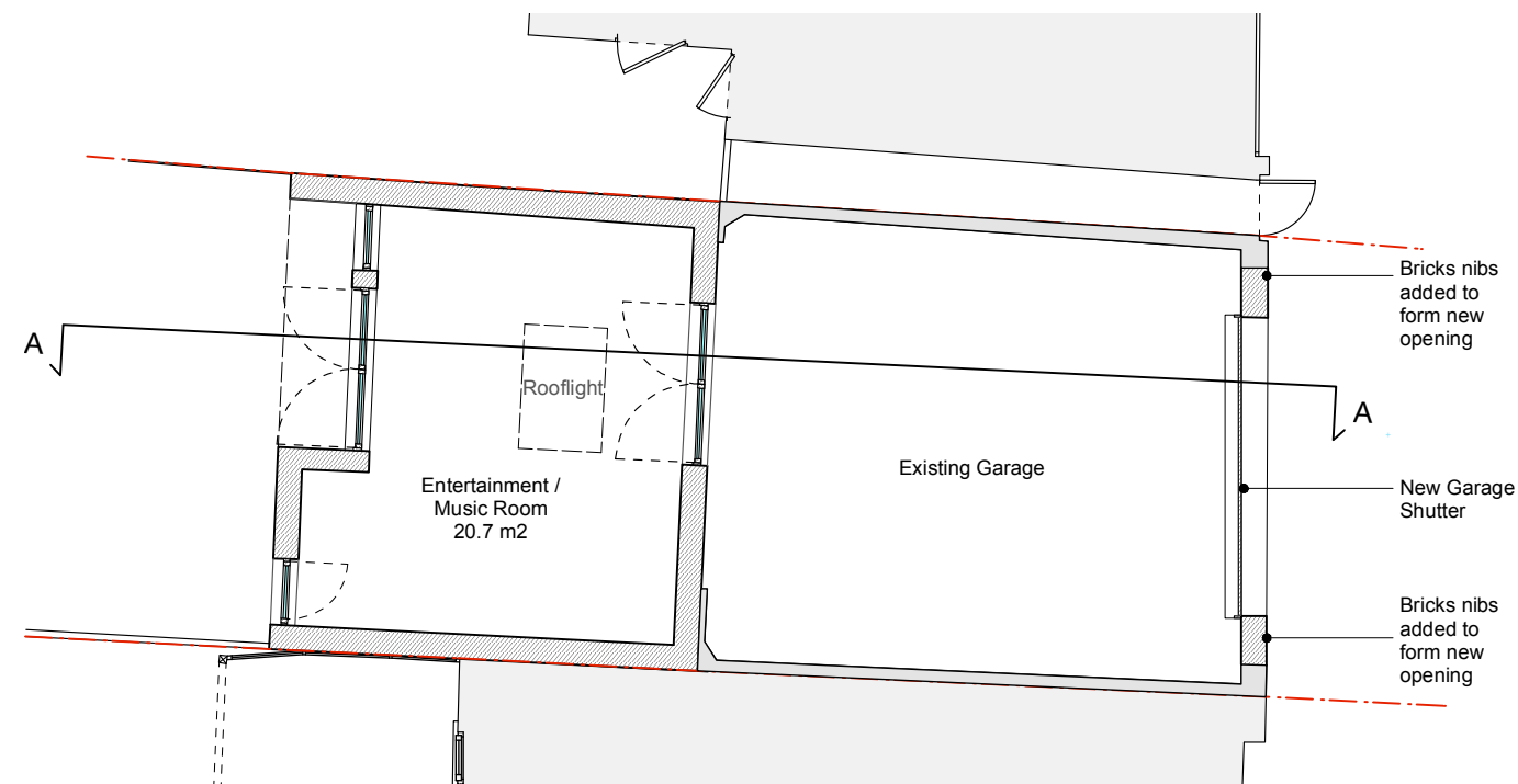
01 - Proposed Outbuilding Plan
