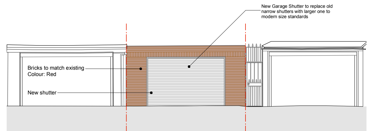
05 - Proposed Street Elevation
