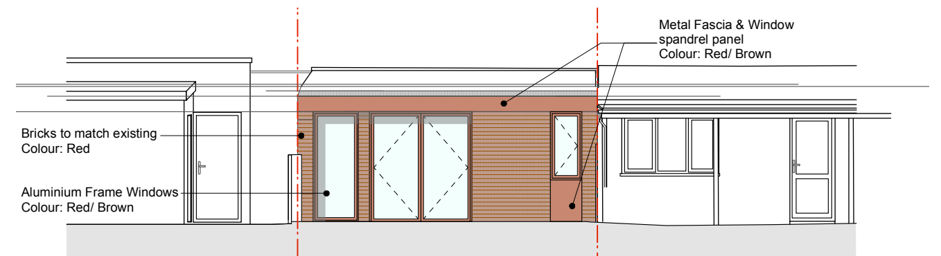
03 - Proposed Garden Elevation
