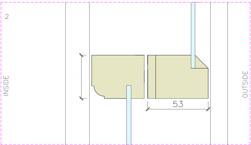
MEETING RAIL SECTION
