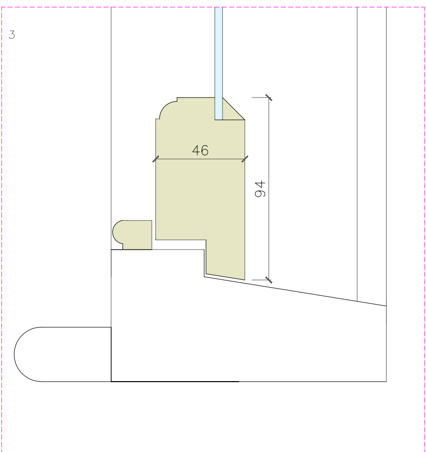
BOTTOM RAIL & SILL SECTION
