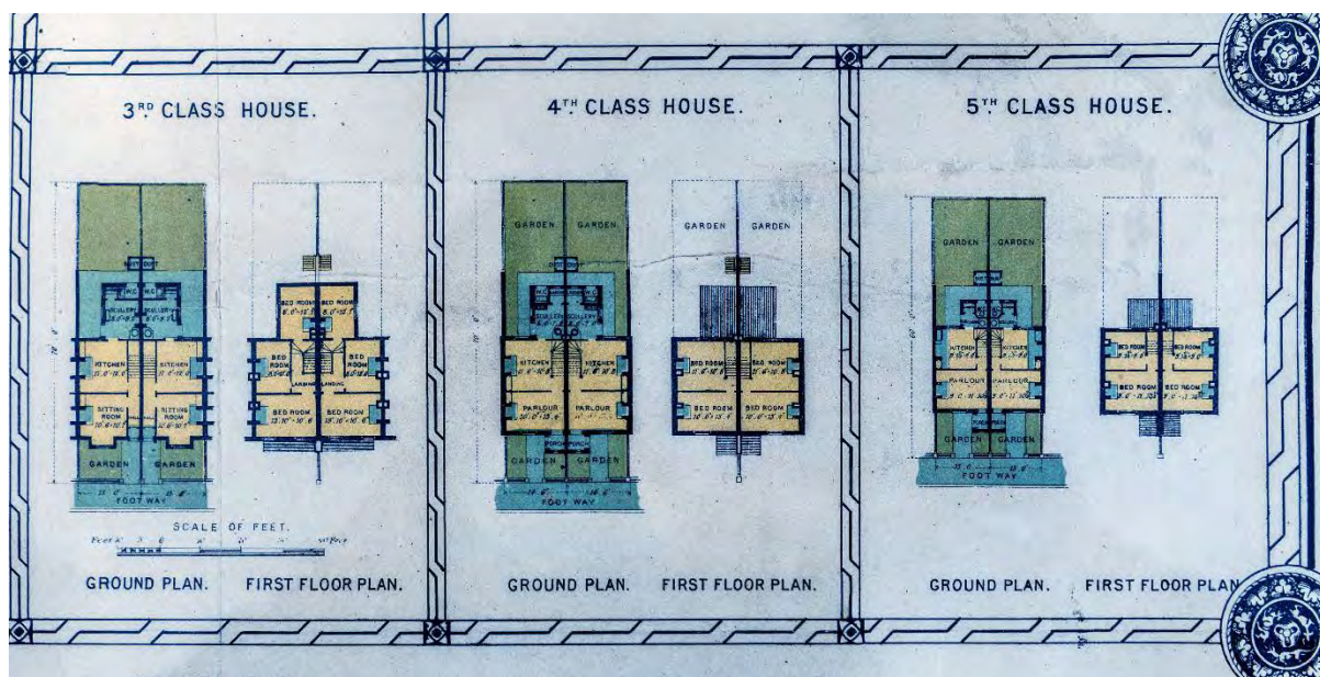
Figure 18 The original plans showing the different types of houses in the Noel Park Estate.
