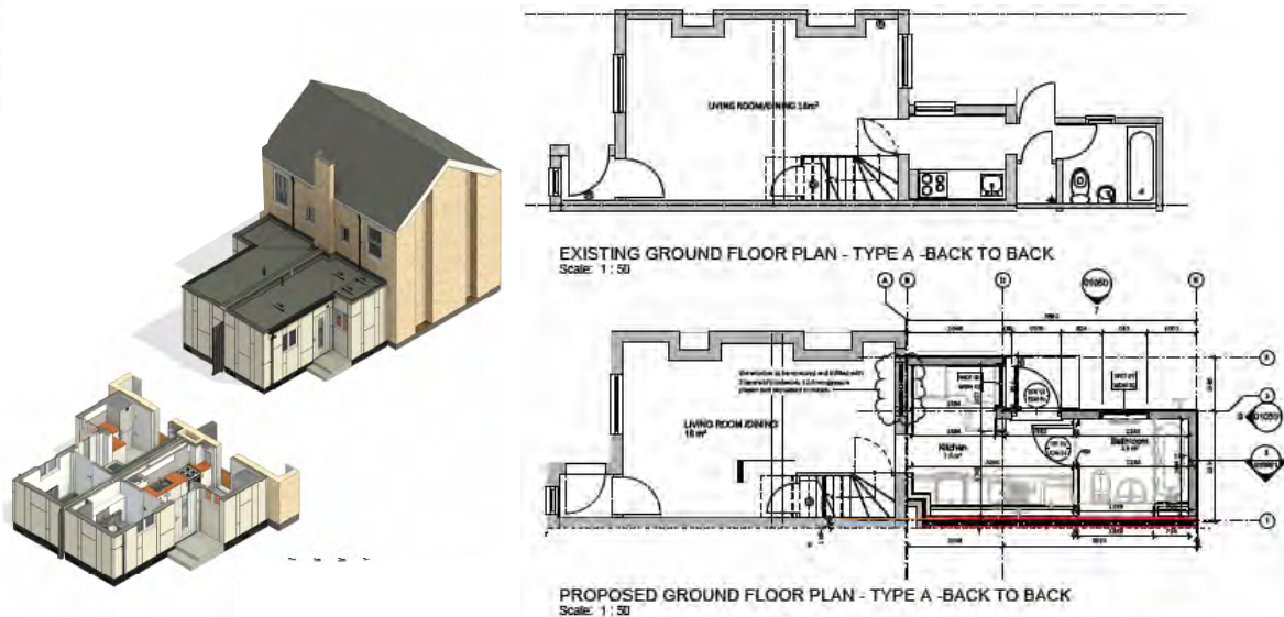
Figure 50: Proposed Pod (Archetype A B2B) and (Above) Existing and proposed plans of No. 209 Moselle Avenue (source: Modulac Wise drawings)
