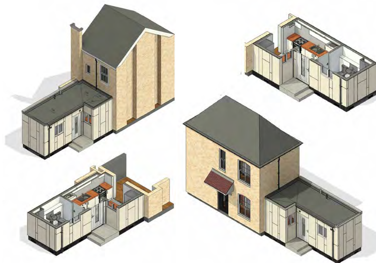
Figure 39: Proposed rear extensions- Archetype A (left) and Archetype BH (right)
