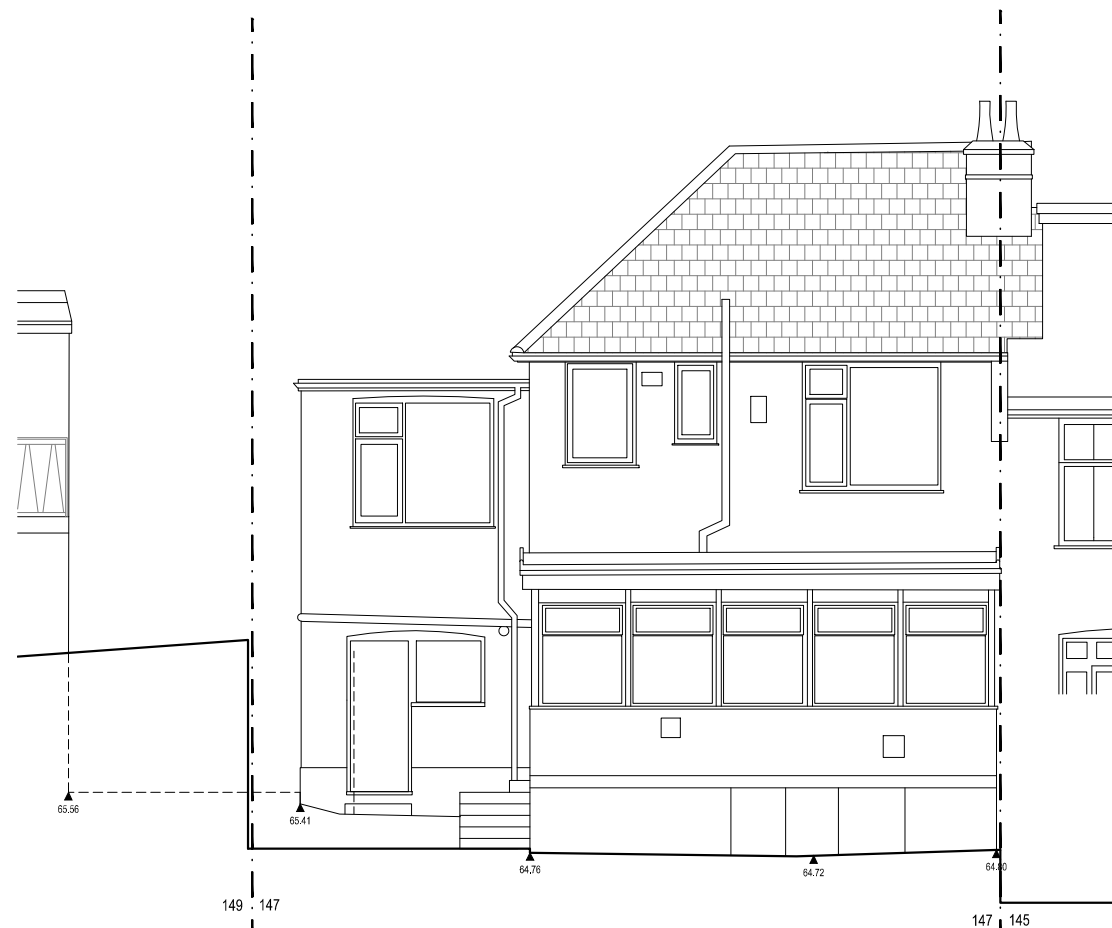
REAR ELEVATION
