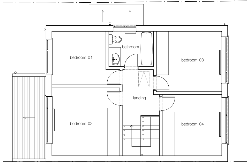
2 first floor plan
