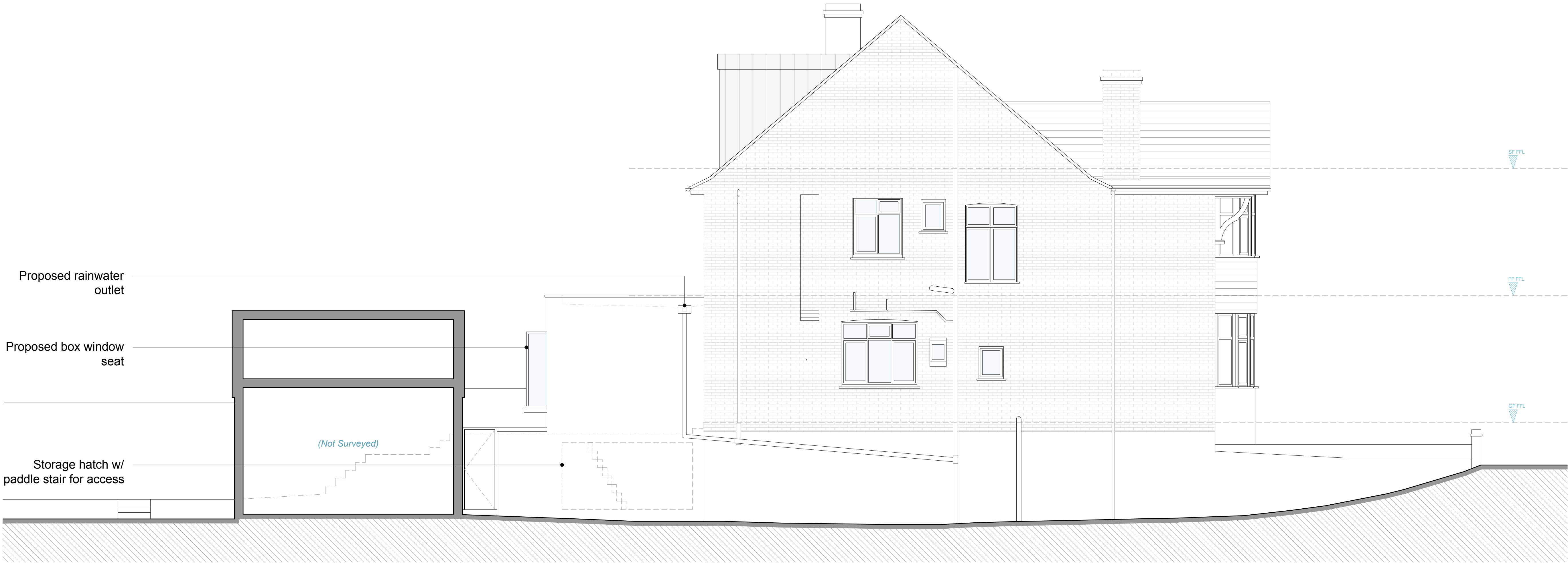
PROPOSED SIDE ELEVATION
