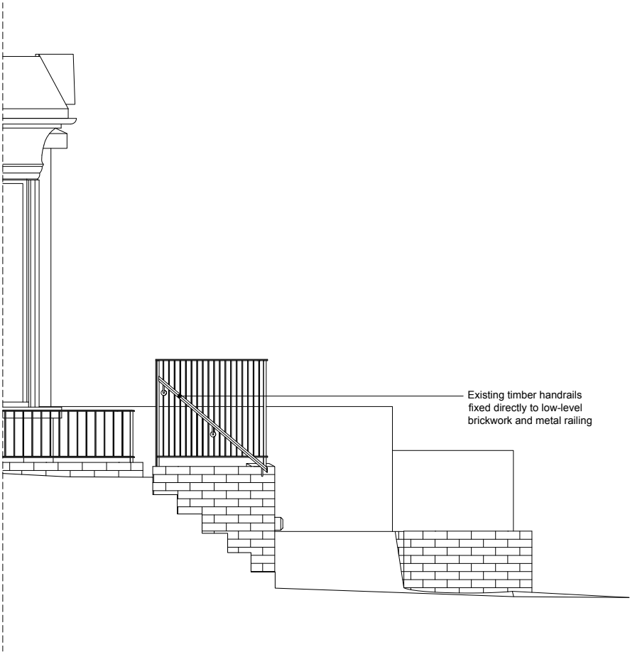
Existing Entrance Handrail - Elevation
