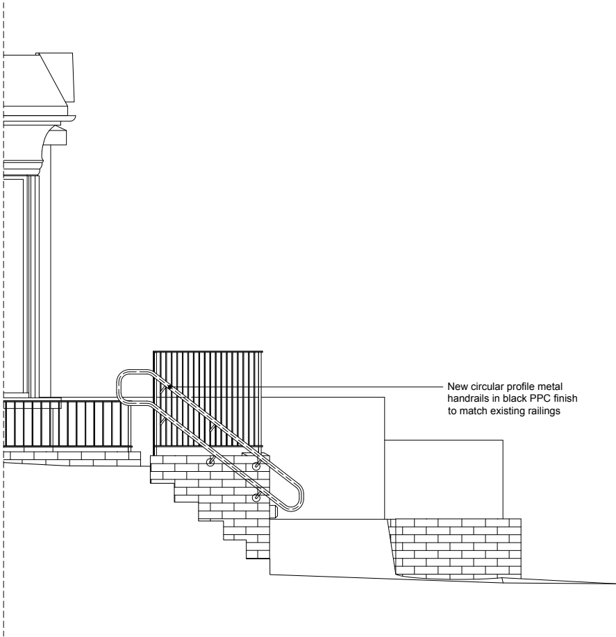
Proposed Entrance Handrail - Elevation
