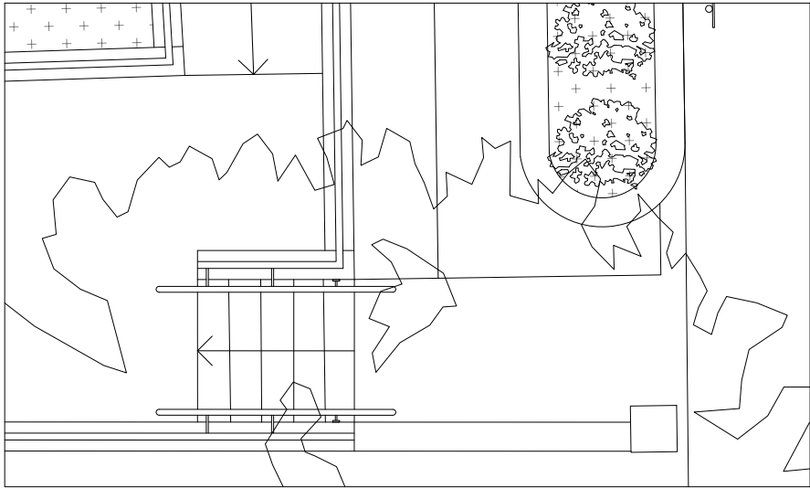
Proposed Entrance Handrail - Plan
