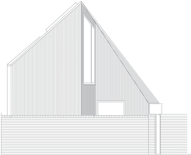
PLANNING APPROVED (HGY/2018/3294) SOUTH-EAST ELEVATION AA 1:100 @A3
