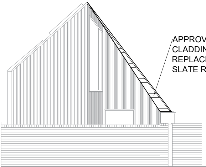
PROPOSED SOUTH EAST ELEVATION AA 1:100 @A3
