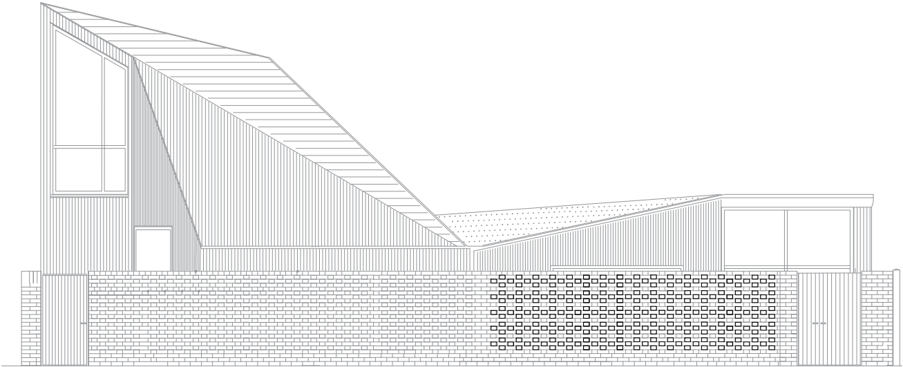
PLANNING APPROVED (HGY/2018/3294) SOUTH-WEST ELEVATION BB 1:100 @A3
