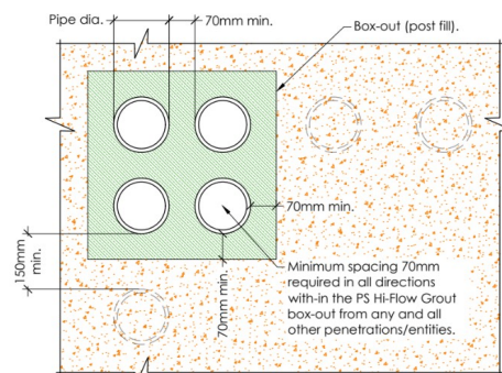
③ Penetration Spacing Detail Scale: 1:10
