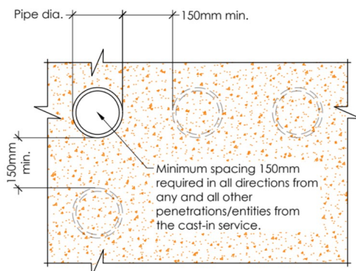
③ Penetration Spacing Detail Scale: 1:10
