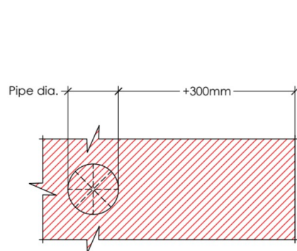
② Membrane Patch Detail Scale: n/a
