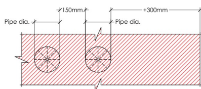
② Box-out Penetration Detail Scale: nts
