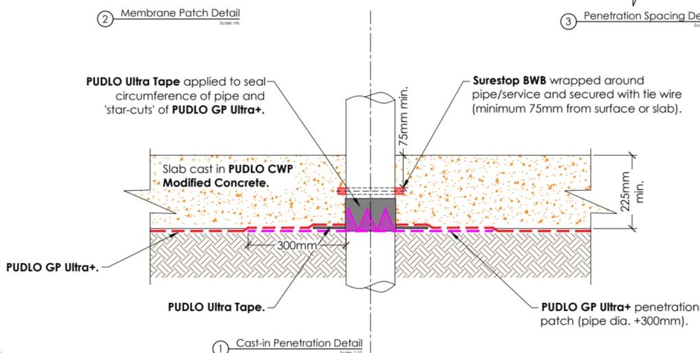
① Cast-in Penetration Detail Scale: 1:10
