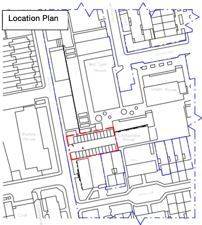
1 Location Plan 1 : 1250
