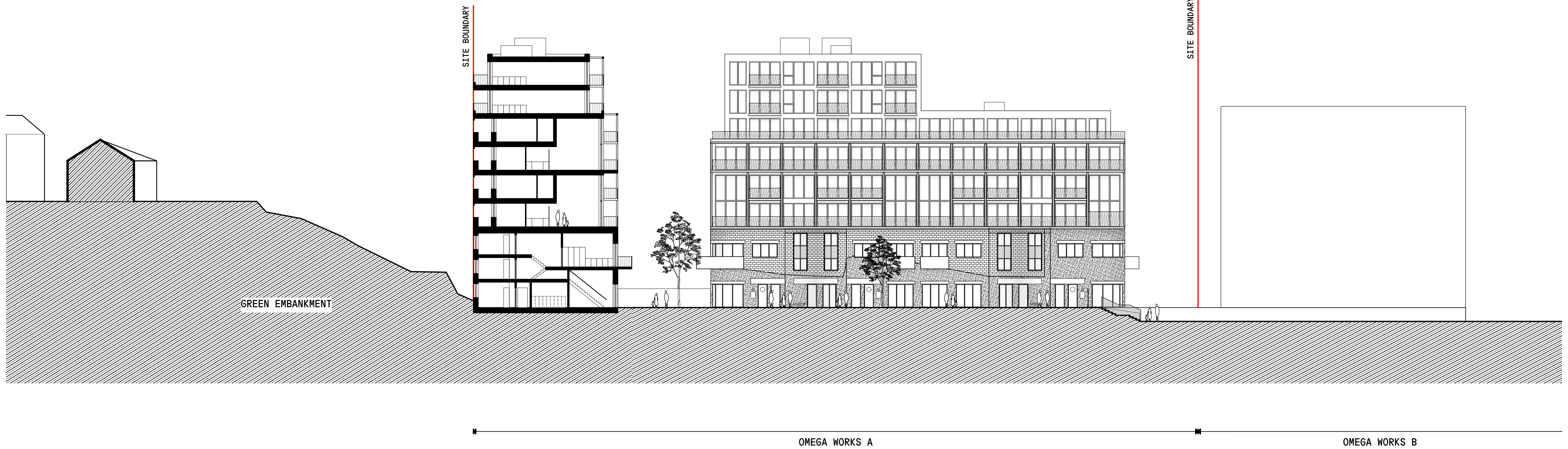
2 PROPOSED CONTEXT SECTION BB SCALE: 1:250
