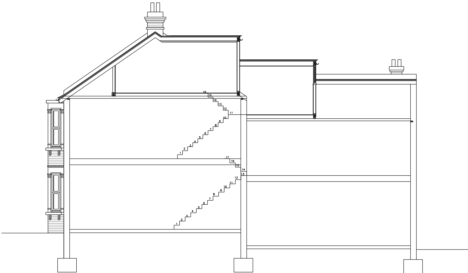
Approved Side Elevation/Section
