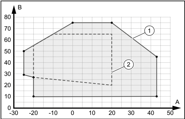
A Outdoor temperature B Heating water temperature 1 Application limits, heating mode 2 Area of application, in accordance with EN 14511
