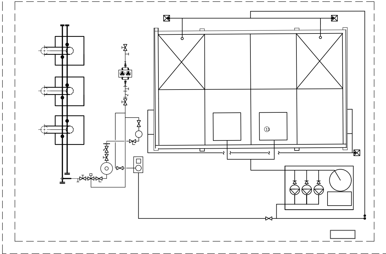
Proposed Plant Enclosure Plan 1:50
