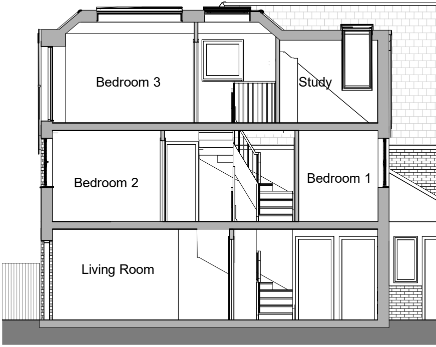
4 Proposed Section 4 1:100
