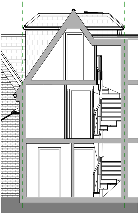
2 Proposed Section 2 1:100
