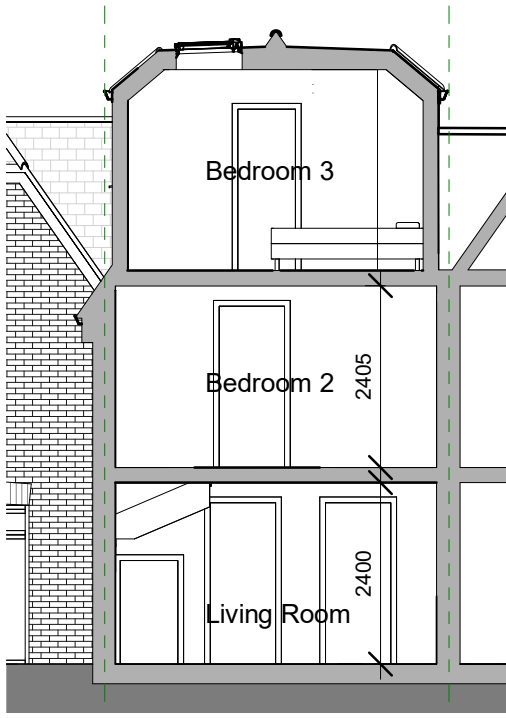
3 Proposed Section 3 1:100
