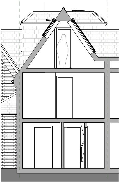
1 Proposed Section 1 1:100
