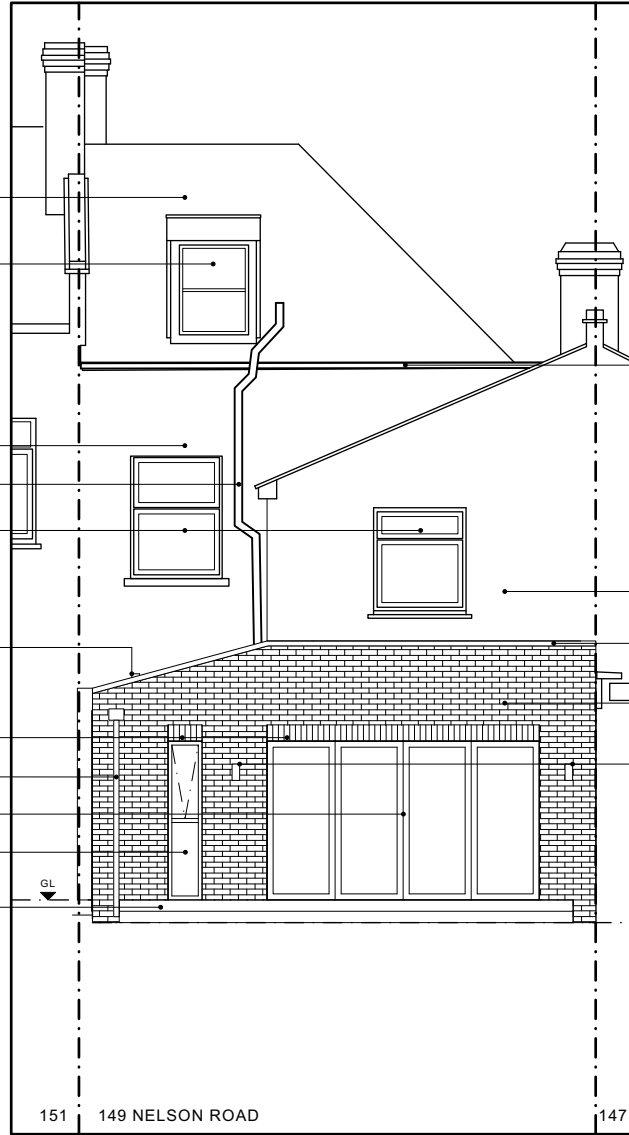
02/2224_PA_PR_300 PROPOSED REAR ELEVATION 1:100 @ A3
