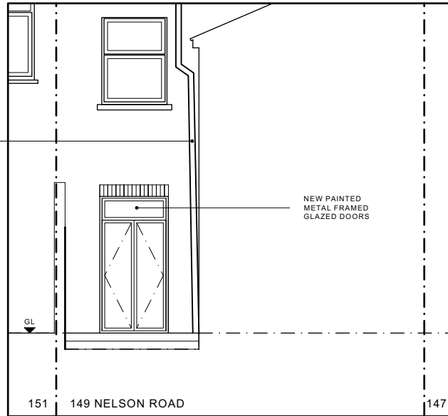
05/2224_PA_PR_300 PROPOSED REAR ELEVATION 1:100 @ A3
