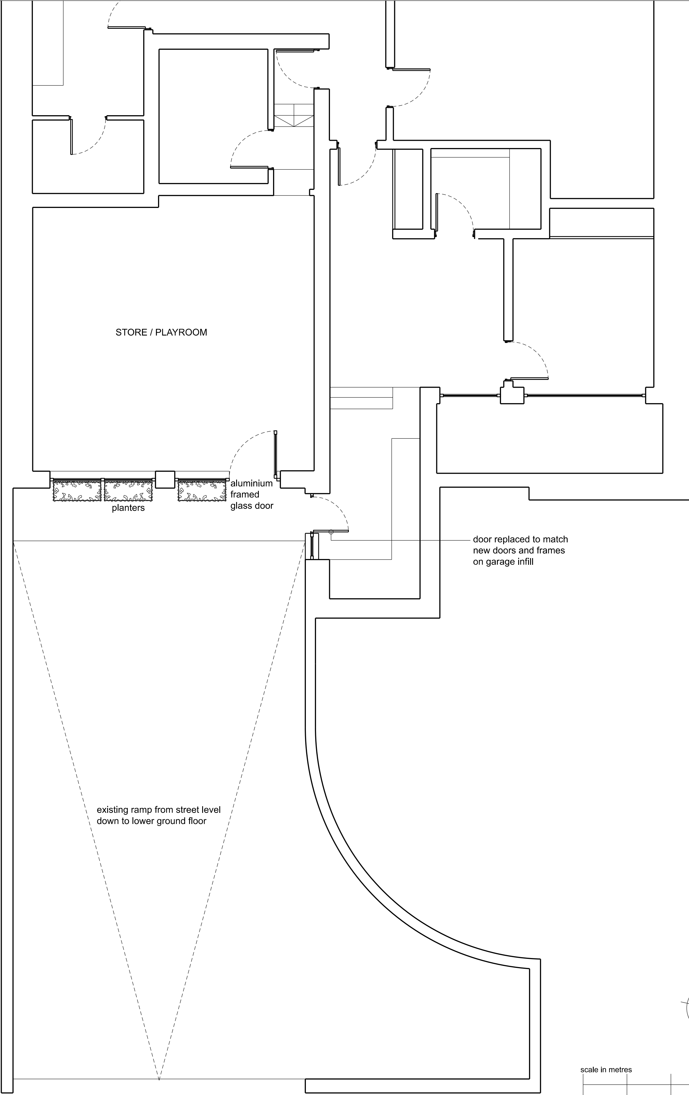
PROPOSED (part) LOWER GROUND FLOOR PLAN
