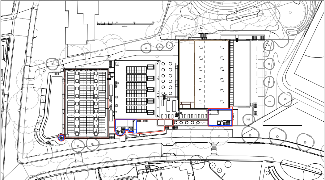
Second Floor Plan level 2 proposed 1:1250 @ A3
