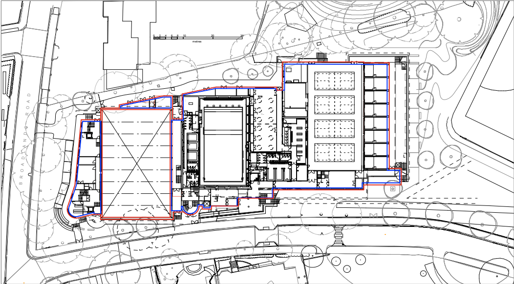
Ground Floor Plan level 0 proposed 1:1250 @ A3
