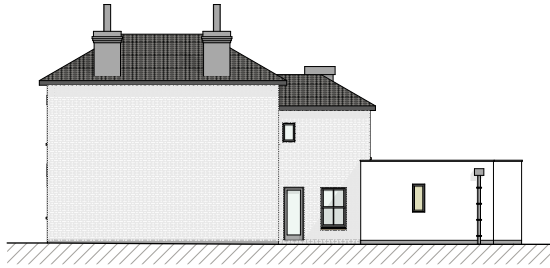
1:100 Side Elevation
