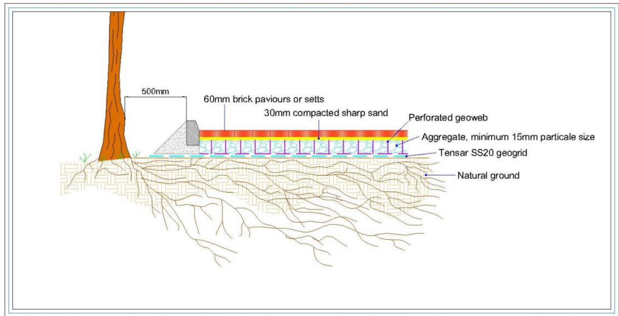
Figure 7: Typical cross-section for multi-dimensional confinement system using kerb edging
