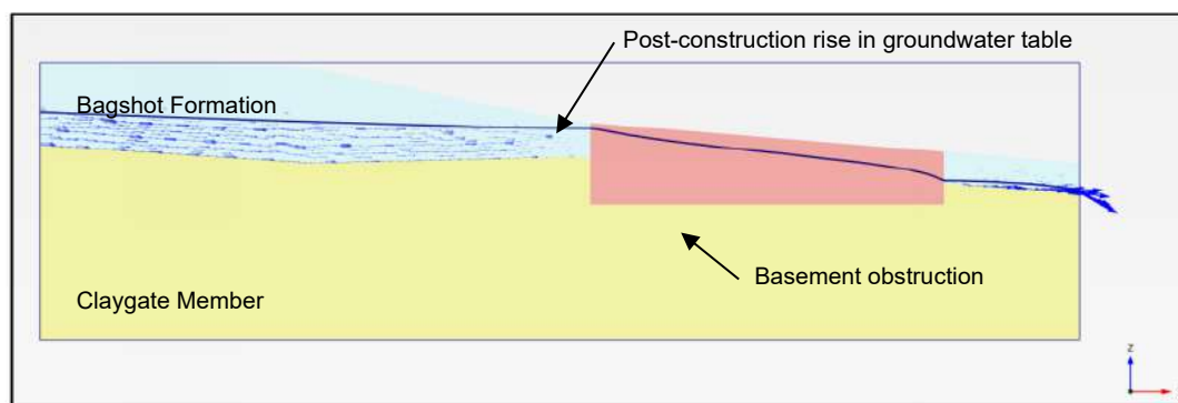
(b) Post-construction groundwater table elevation
