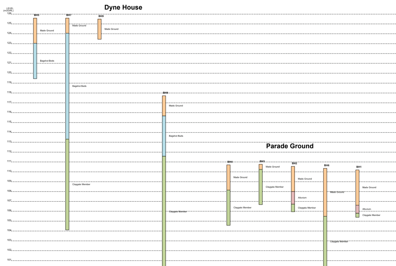
Figure 5.2: Indicative cross-section through site-specific boreholes (west to east)
