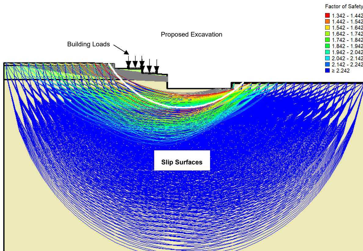
Figure 6.2: Indicative plot of the slip surfaces assessed in GeoStudio SLOPE for the slope following the proposed works on the Dyne House plot
