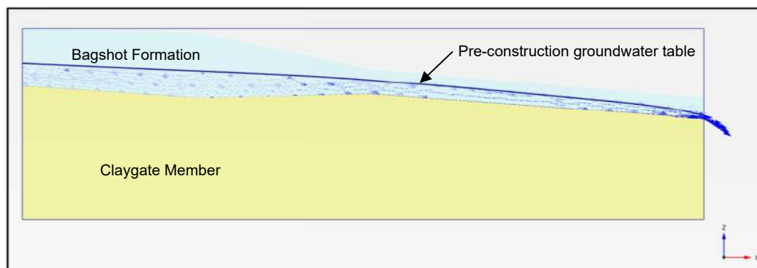
(a) Pre-construction groundwater table elevation
