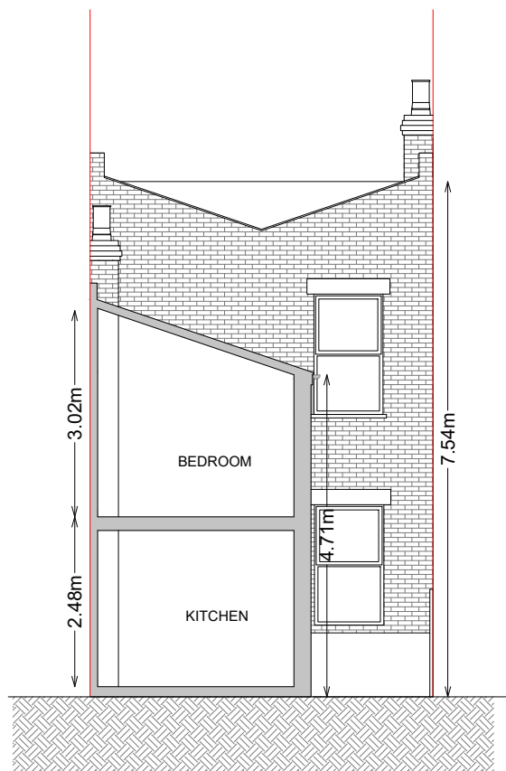
EXISTING SECTION A-A scale 1:100
