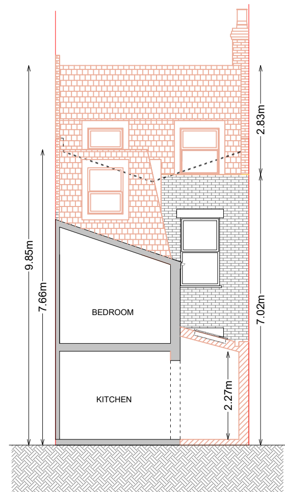
PROPOSED SECTION A-A scale 1:100
