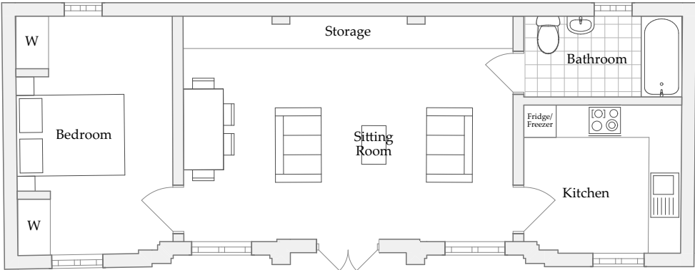
Proposed Floor plan
