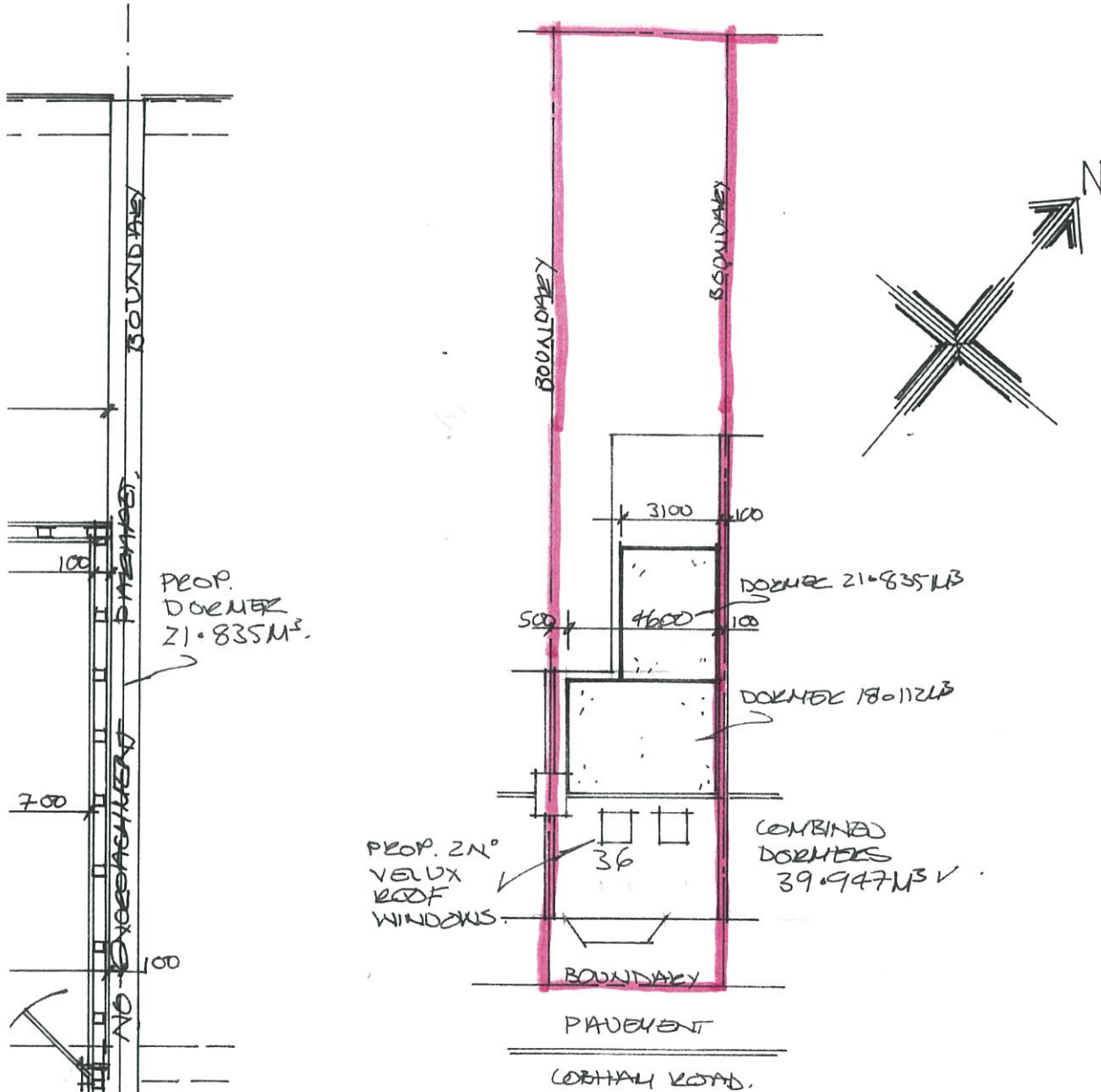
Prop. Block Plan.
