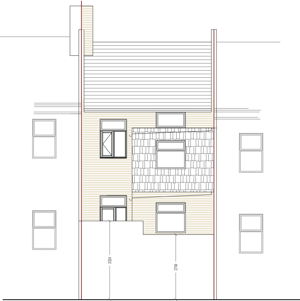
scale 1:100 0m 1m 2m 3m 4m 5m Rear Elevation - Existing
