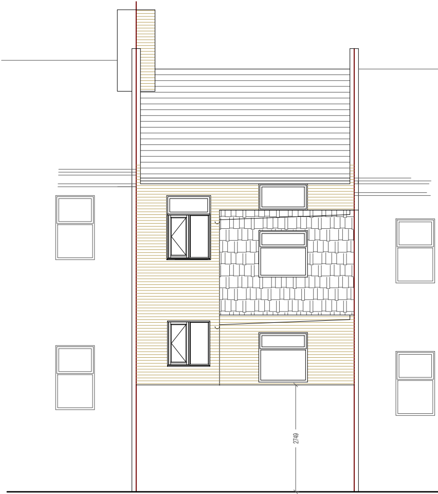
scale 1:100 0m 1m 2m 3m 4m 5m Rear Elevation - Existing
